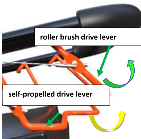
Fig.29-1 Pull rod closing direction
