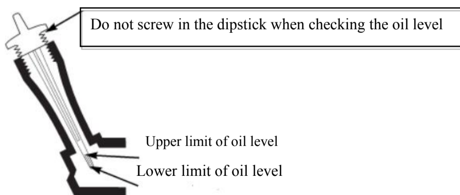
Fig.39-2 Measuring oil level
